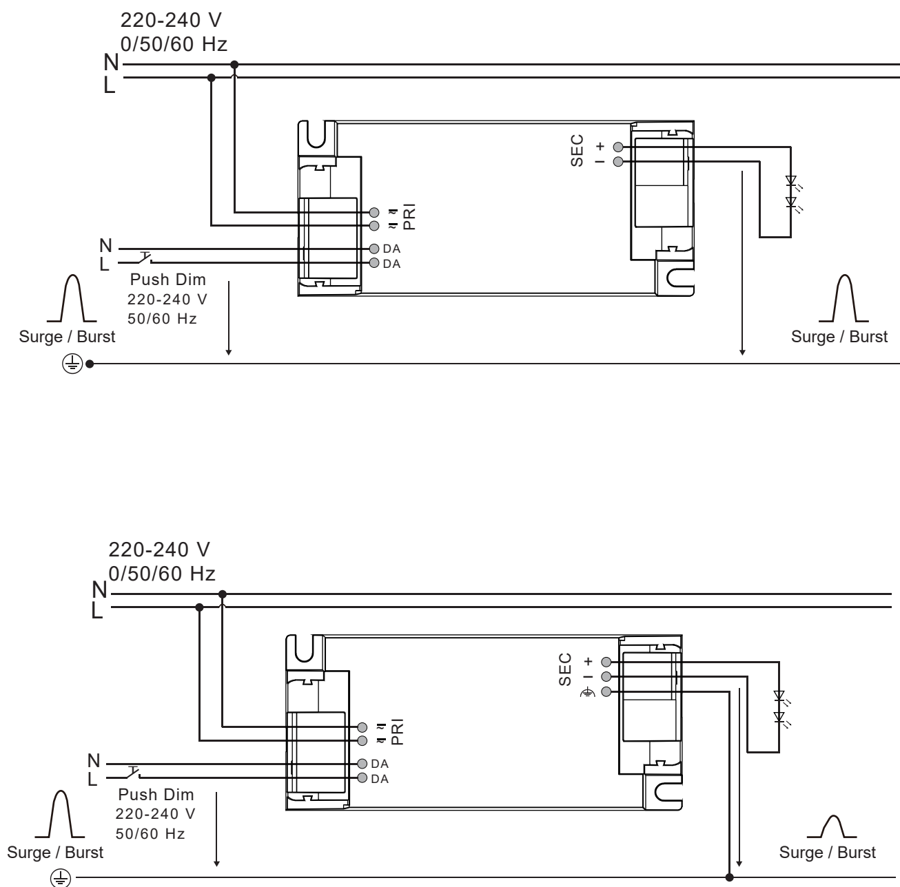
Figure: Voltage peaks for LED driver without earthing (Above) and with earthing (Below)
